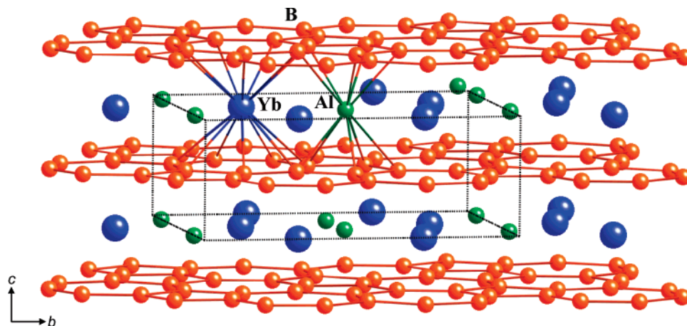
Figure 1. Layers of \beta\text{-YbAlB}_4 . Boron, shown as orange spheres, forms two-dimensional sheets along the ab -plane. Layers of Yb, shown in blue, and Al, shown in green, are interleaved between the B layers. Dashed lines show the orthorhombic unit cell. Some interlayer bonding has been omitted for clarity.
