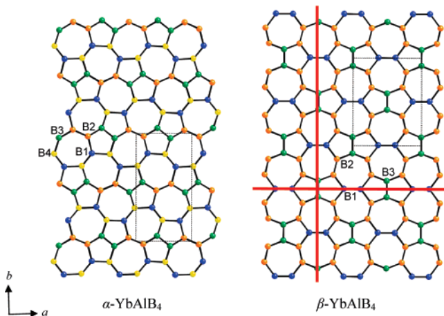
Figure 2. Boron layers along [020] for (a) \alpha\text{-YbAlB}_4 and (b) \beta\text{-YbAlB}_4 . The unit cell is outlined with grey lines. For \alpha\text{-YbAlB}_4 , the B1, B2, B3, and B4 atoms are shown as blue, orange, green, and yellow spheres, respectively. For \beta\text{-YbAlB}_4 , the B1, B2, and B3 atoms are shown as blue, orange, and green spheres, respectively. Mirror planes are depicted as solid red lines.
